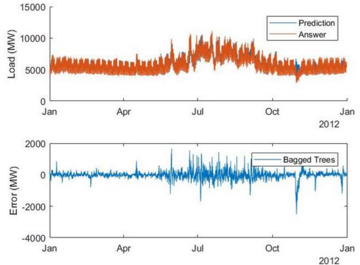
Figure 3. Validation results of an AI model that is predicting load consumption plotted using MATLAB. a) Bagged tree-based regression model with the predicted data plotted against actual consumption data. b) Error between predicted data and actual consumption data.
